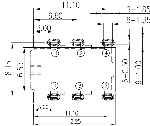
RECOMMEND PCB LAYOUT TOLERANCE :±0.05
