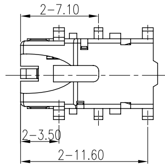
PLUG SPEC
